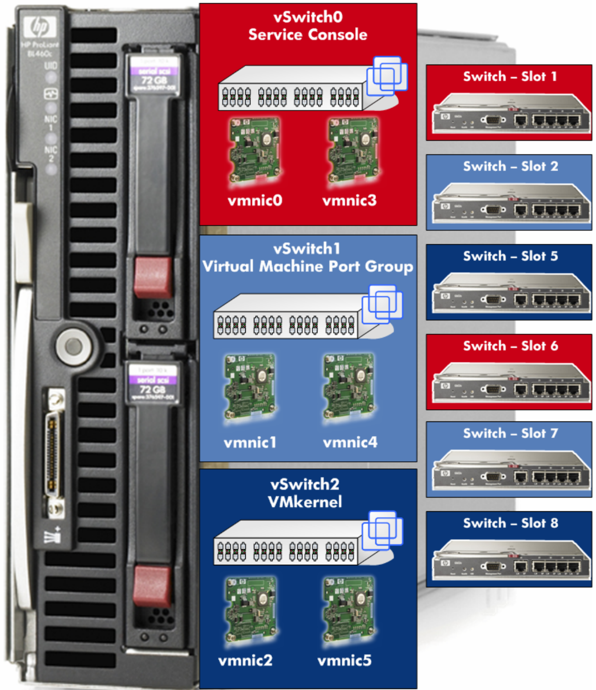
Figure 3. This graphic shows a redundant network configuration for the suggested reference configuration, including virtual switches.
